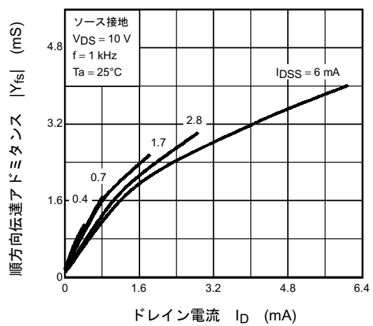
|Yfs| - ID
