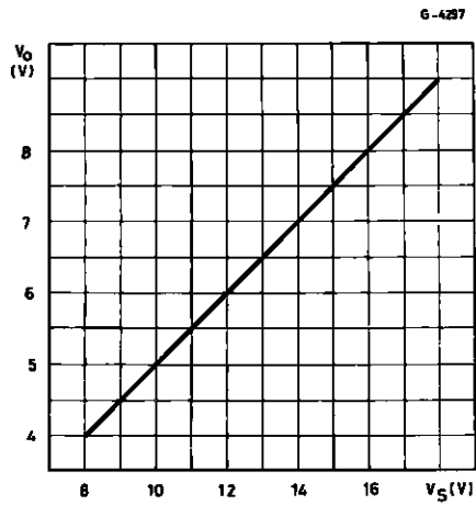
Figure 3 : Quiescent Output Voltage vs. Supply Voltage.
